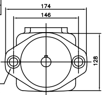
2-#13.5 HOLE #21 SPOTFACER 1 DEEP
