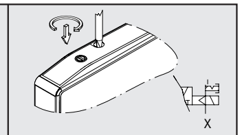
BISTABLE OVERRIDE PORT 4 servo-assisted
