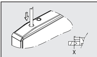
MONOSTABLE OVERRIDE PORT 2 with direct actuation on the spool
