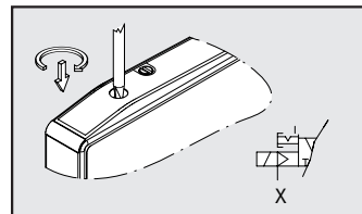
BISTABLE OVERRIDE PORT 2 with direct actuation on the spool
